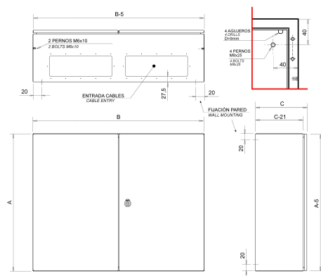
Standard drawing
