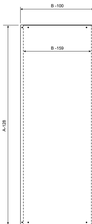
Mounting plate
