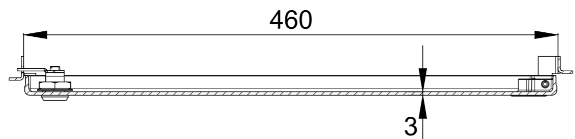
SEC. A-A'
