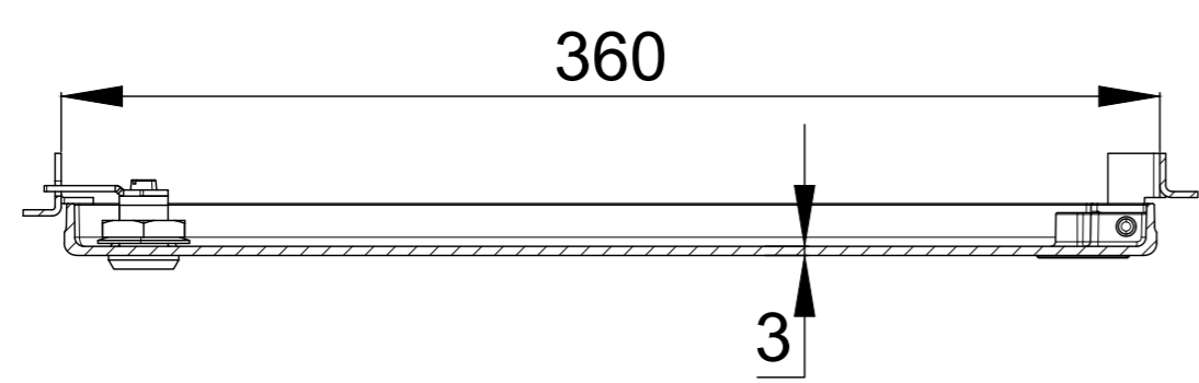
SEC. A-A'
