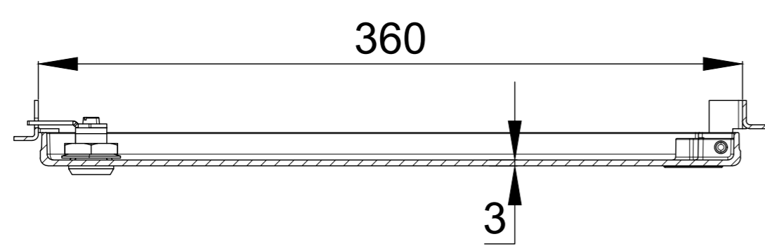
SEC. A-A'
