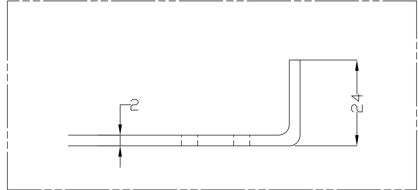
SEC. B-B
