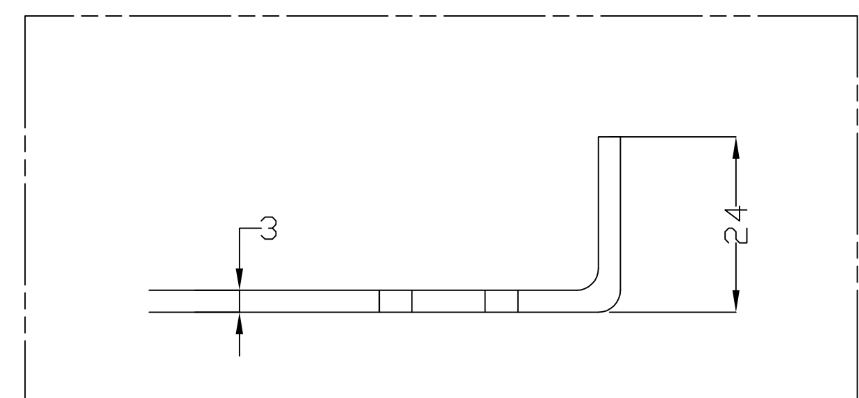
SEC. B-B
