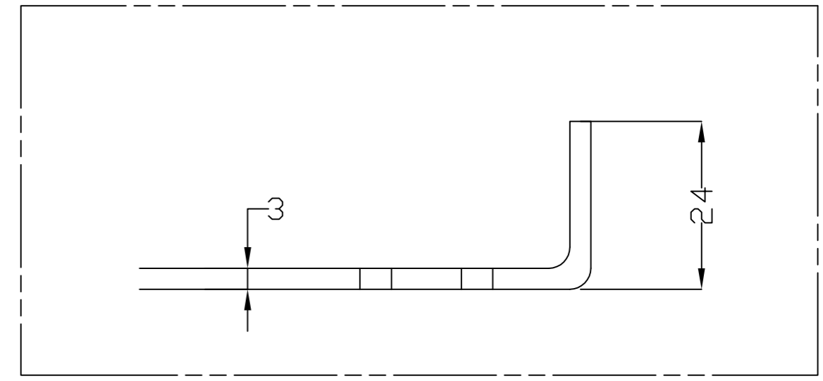
SEC. B-B
