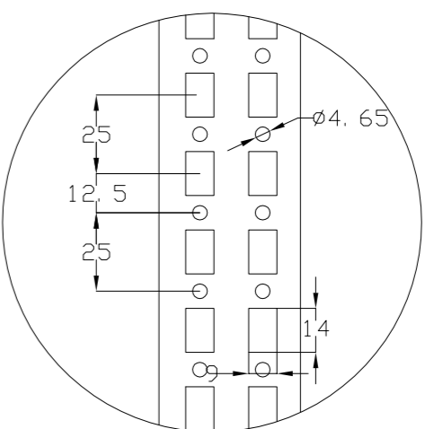
DETALLE X X DETAIL
