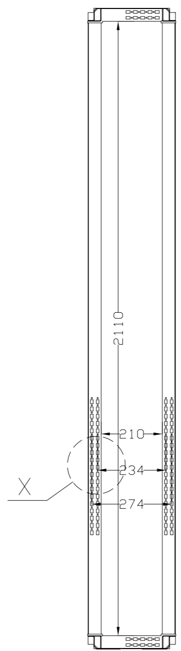
SEC. B-B
