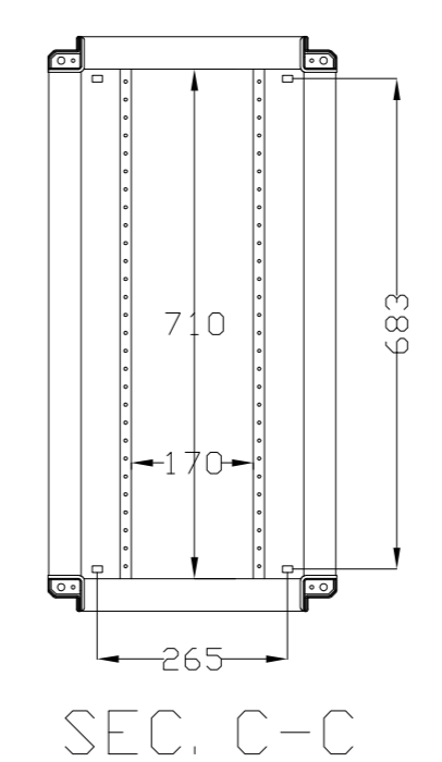
SEC. C-C
