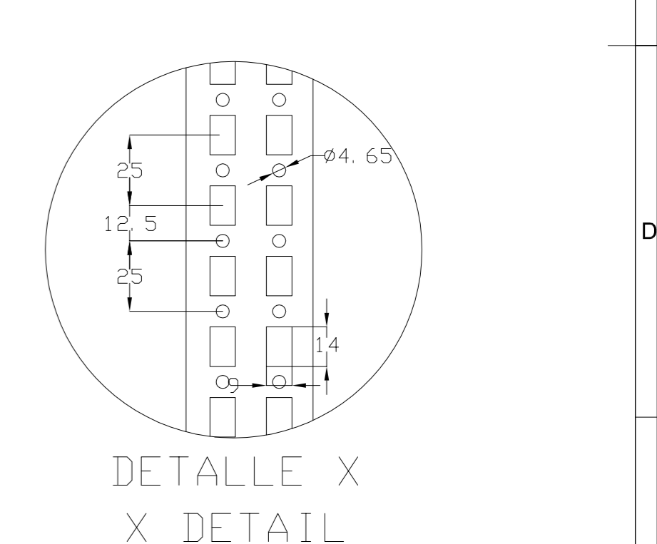
DETALLE X X DETAIL
