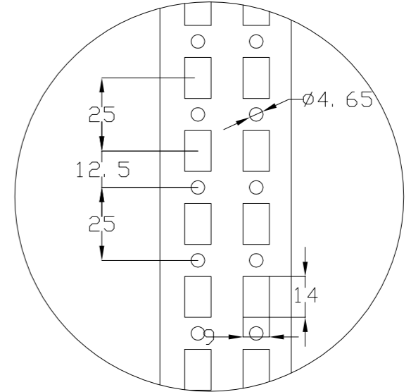
DETALLE X X DETAIL
