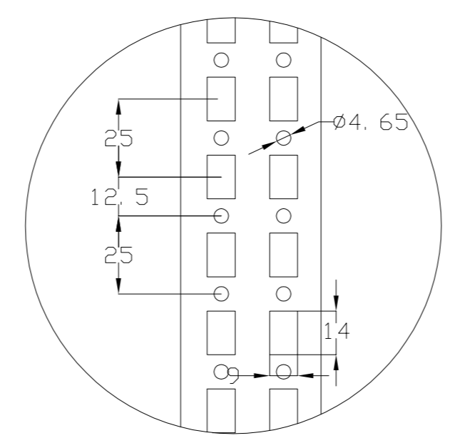
DETALLE X X DETAIL
