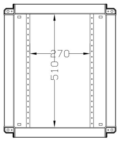
SEC. C-C
