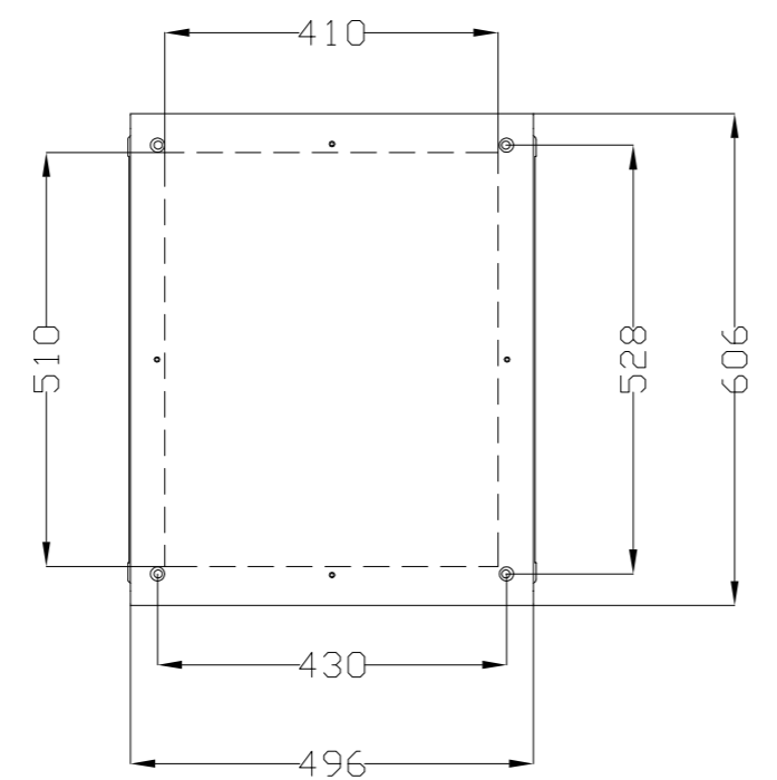
VISTA SUPERIOR TOP VIEW
