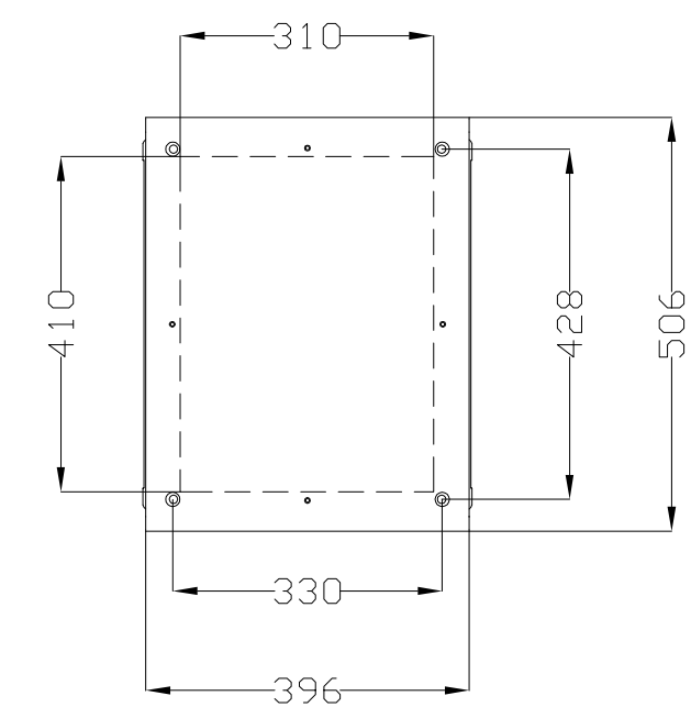
VISTA SUPERIOR TOP VIEW
