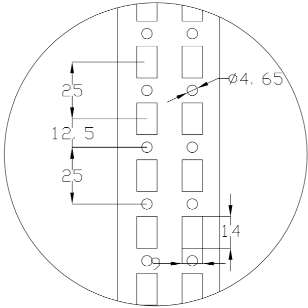
DETALLE X X DETAIL
