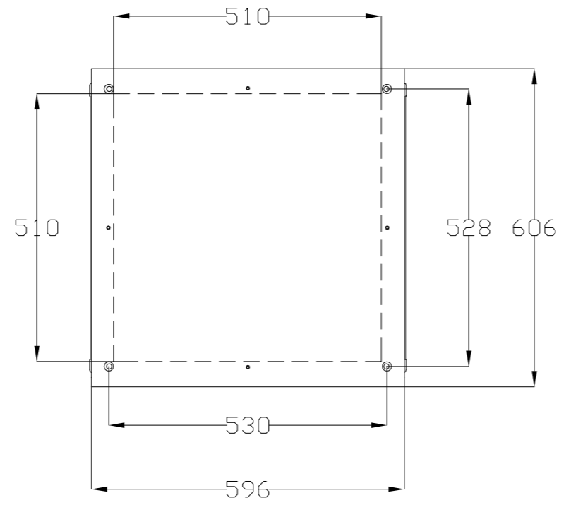
VISTA SUPERIOR TOP VIEW
