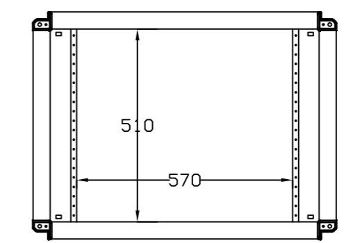
SEC. C-C
