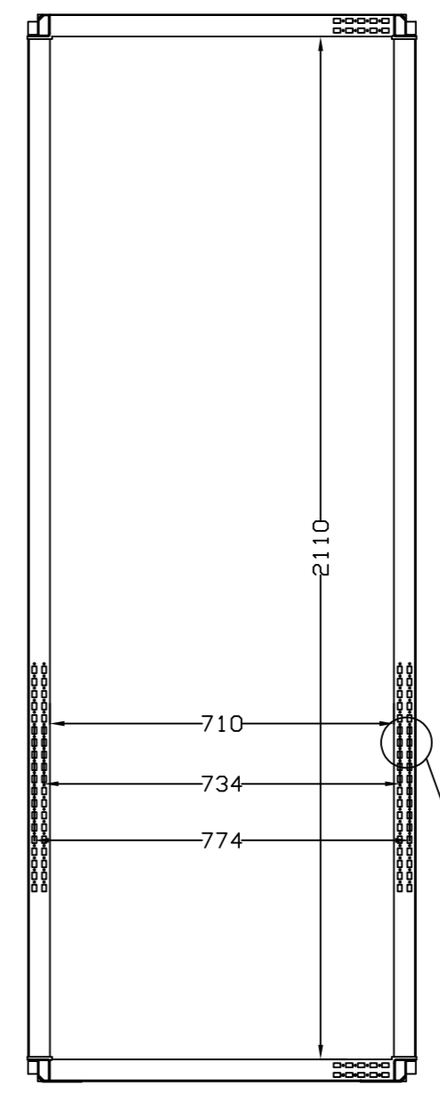
SEC. B-B
