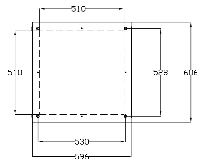
VISTA SUPERIOR TOP VIEW
