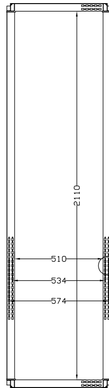
SEC. B-B
