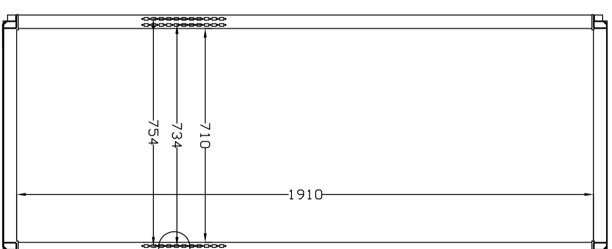
SEC. B-B
