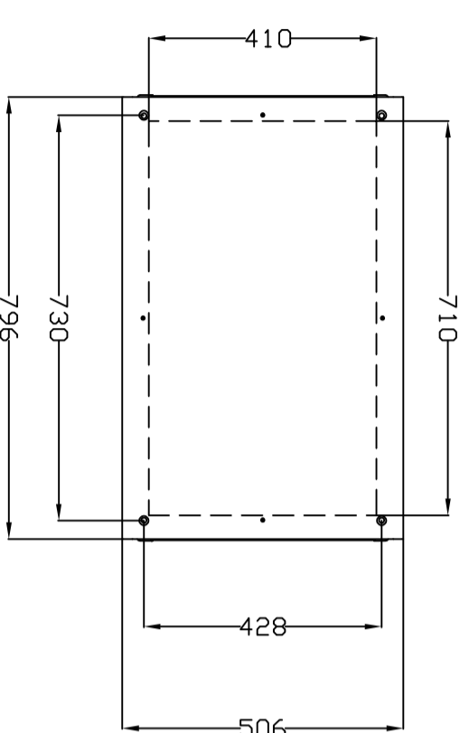
VISTA SUPERIOR TOP VIEW
