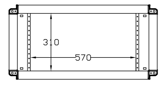
SEC. C-C
