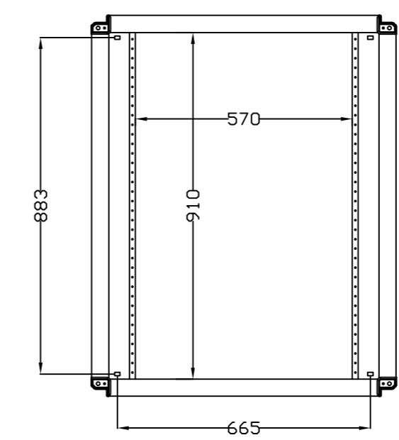
SEC. C-C
