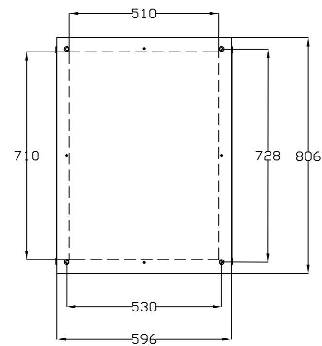
VISTA SUPERIOR TOP VIEW
