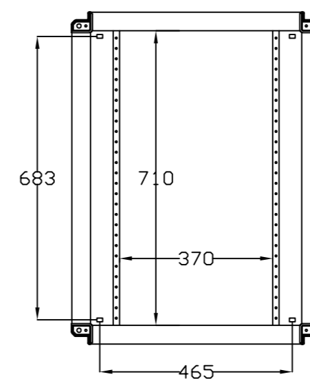
SEC. C-C
