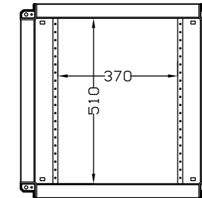
SEC. C-C
