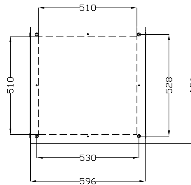
VISTA SUPERIOR TOP VIEW
