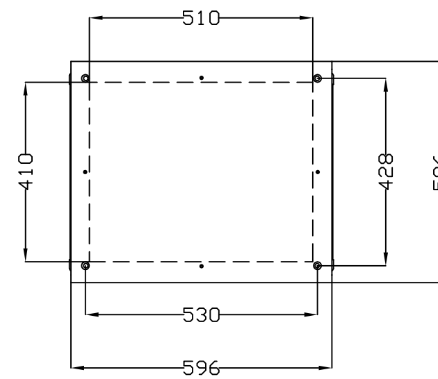
VISTA SUPERIOR TOP VIEW
