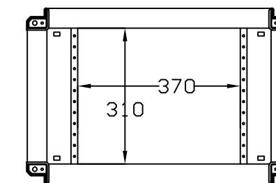
SEC. C-C
