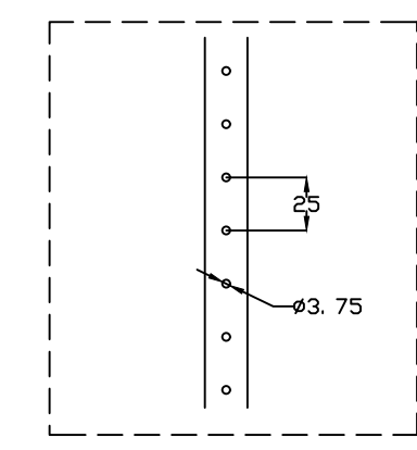
DETALLE X X DETAIL
