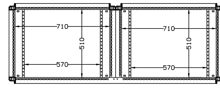
SEC. C-C
