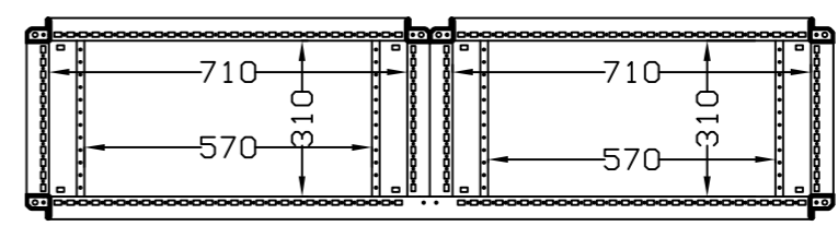
SEC. C-C
