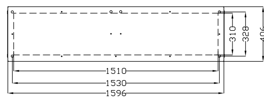
VISTA SUPERIOR TOP VIEW
