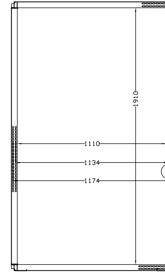
SEC. B-B
