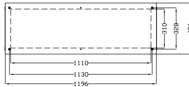
VISTA SUPERIOR TOP VIEW
