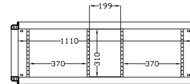
SEC. C-C
