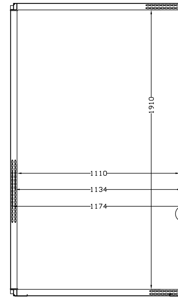
SEC. B-B
