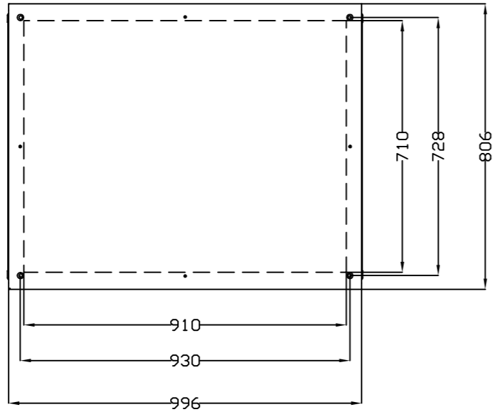
VISTA SUPERIOR TOP VIEW
