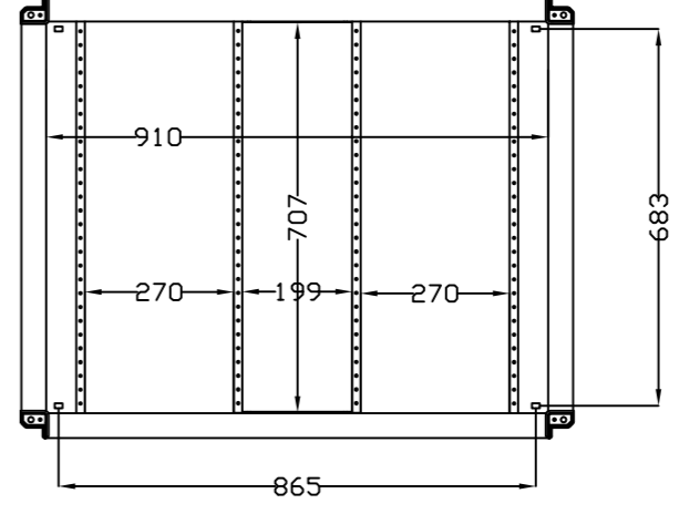
SEC. C-C
