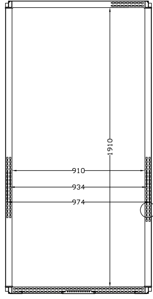
SEC. B-B
