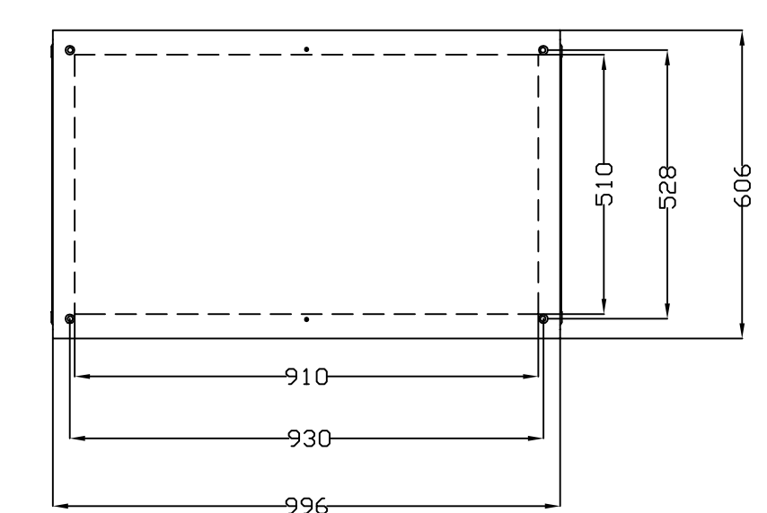
VISTA SUPERIOR TOP VIEW
