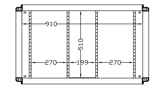
SEC. C-C
