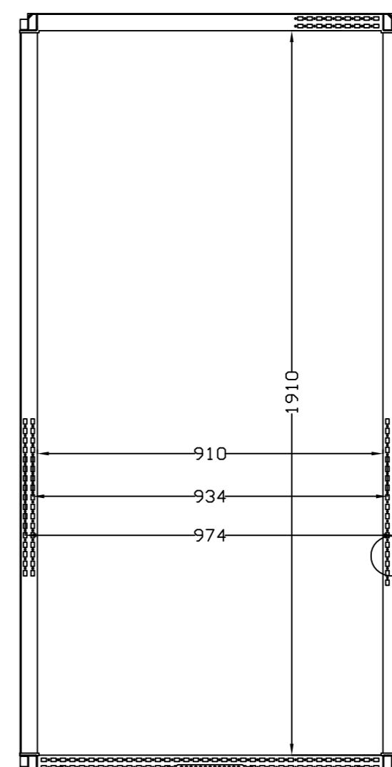
SEC. B-B
