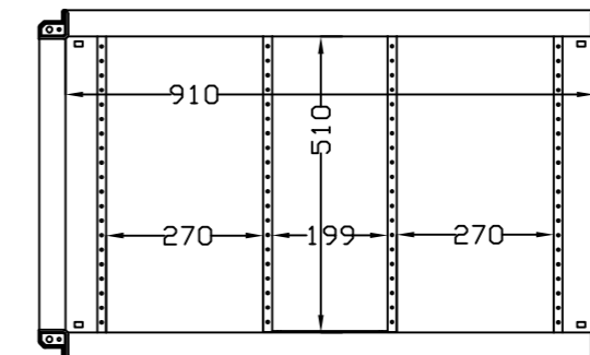
SEC. C-C
