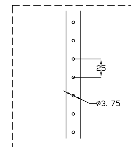
DETALLE X X DETAIL
