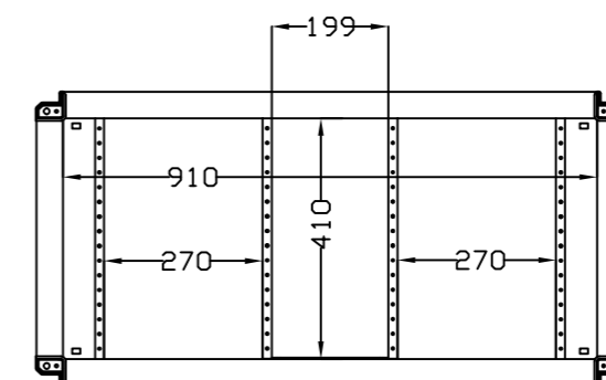
SEC. C-C
