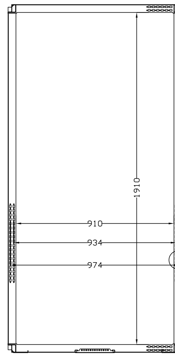
SEC. B-B
