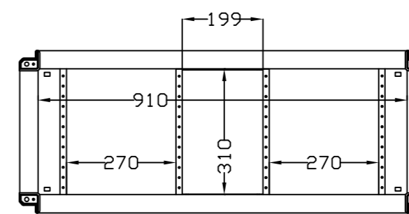
SEC. C-C
