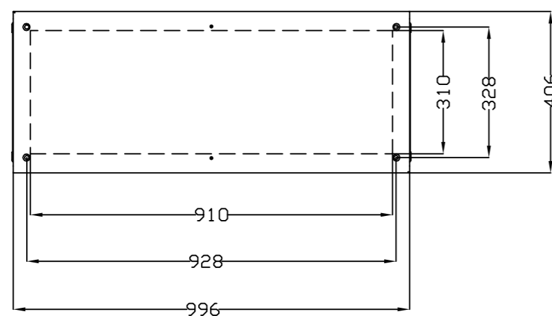
VISTA SUPERIOR TOP VIEW
