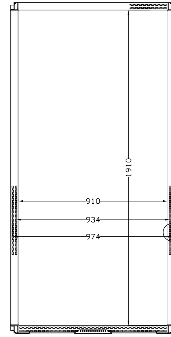
SEC. B-B
