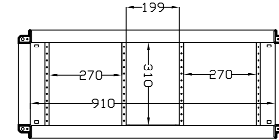
SEC. C-C
