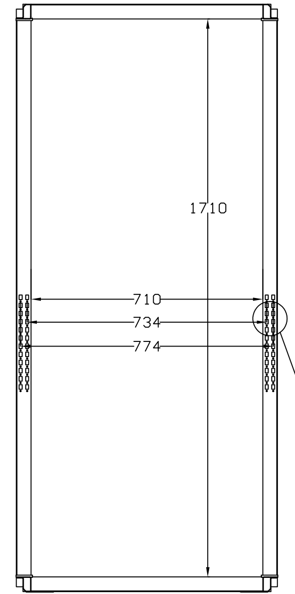
SEC. B-B
