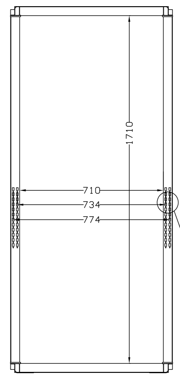
SEC. B-B
