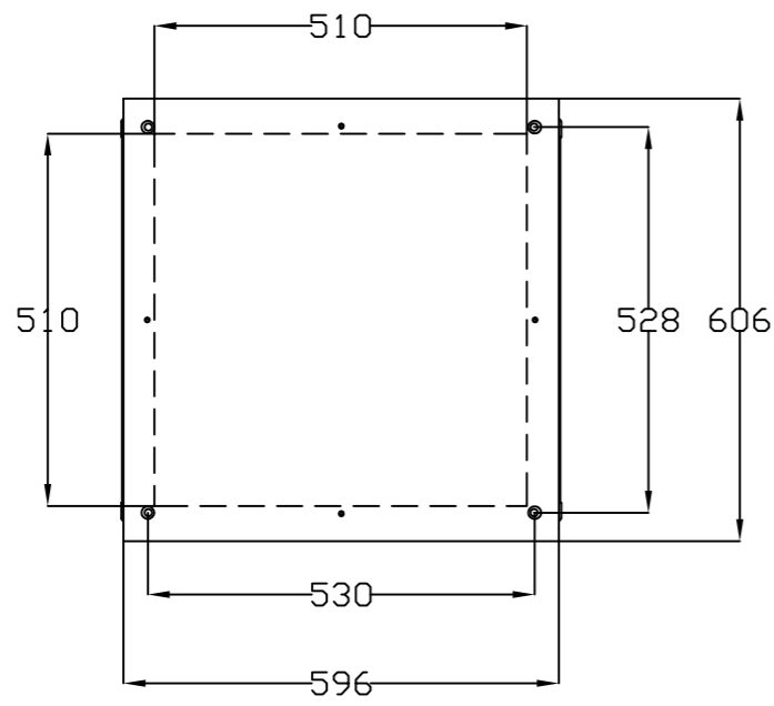
VISTA SUPERIOR TOP VIEW
