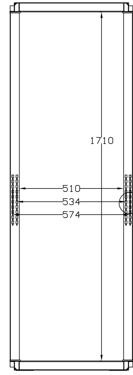
SEC. B-B
