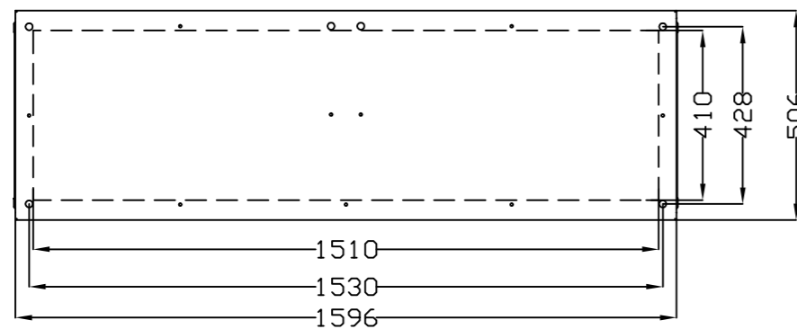
VISTA SUPERIOR TOP VIEW
