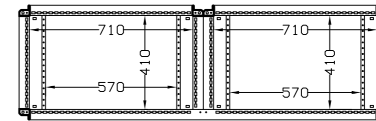
SEC. C-C
