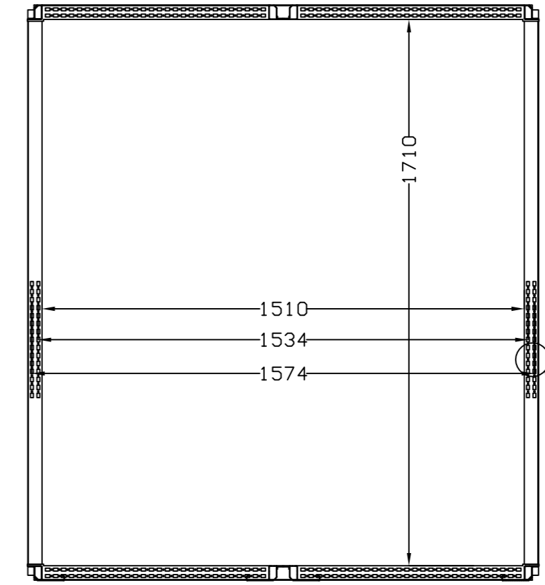
SEC. B-B
