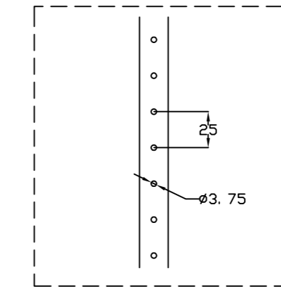
DETALLE X X DETAIL
