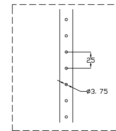
DETALLE X X DETAIL
