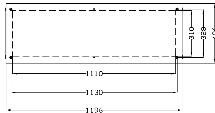
VISTA SUPERIOR TOP VIEW
