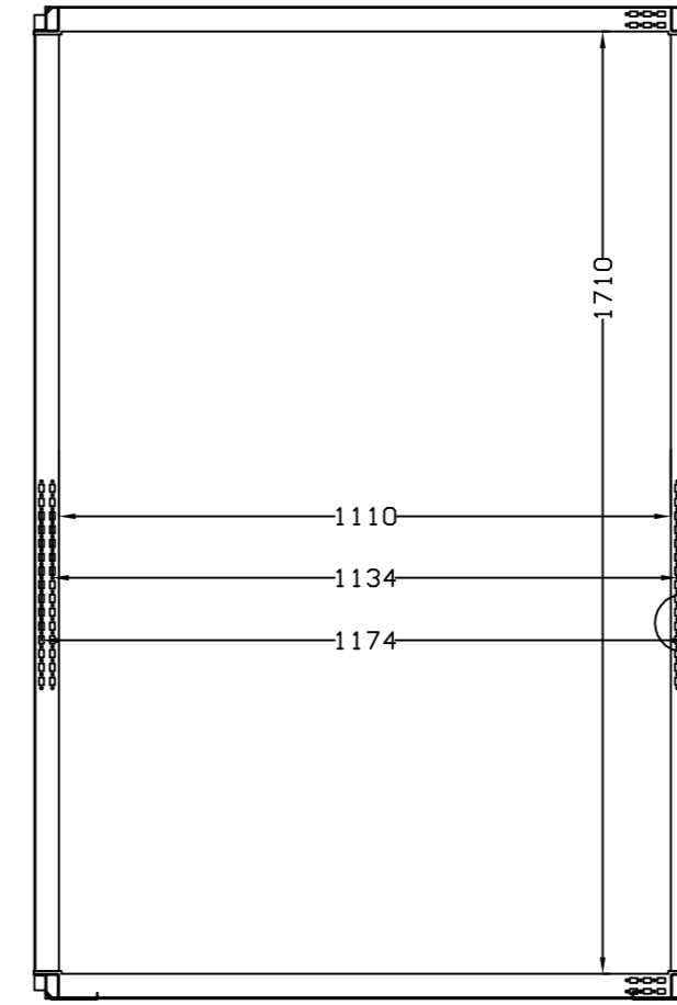
SEC. B-B
