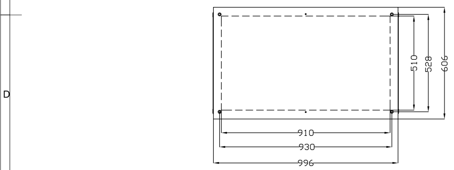
VISTA SUPERIOR TOP VIEW
