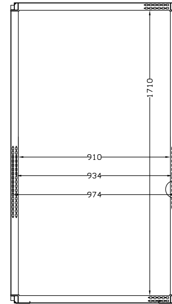
SEC. B-B
