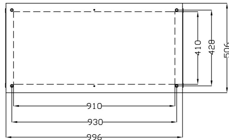
VISTA SUPERIOR TOP VIEW
