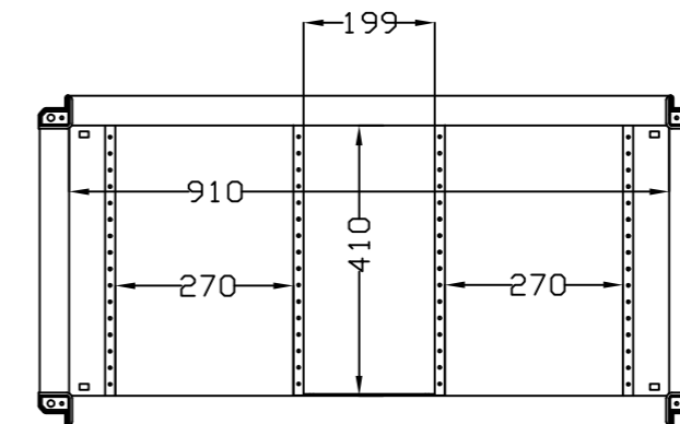
SEC. C-C
