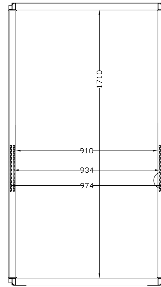
SEC. B-B
