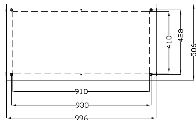
VISTA SUPERIOR TOP VIEW
