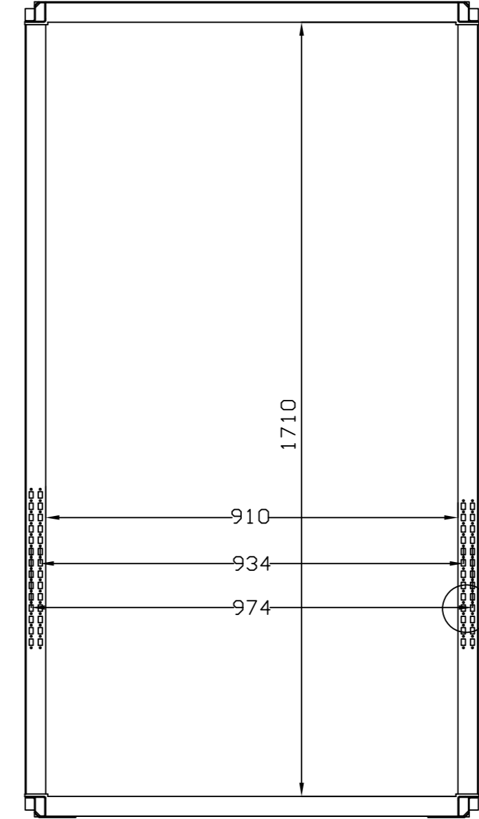
SEC. B-B
