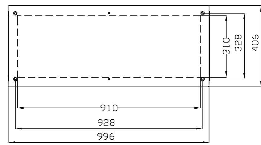
VISTA SUPERIOR TOP VIEW
