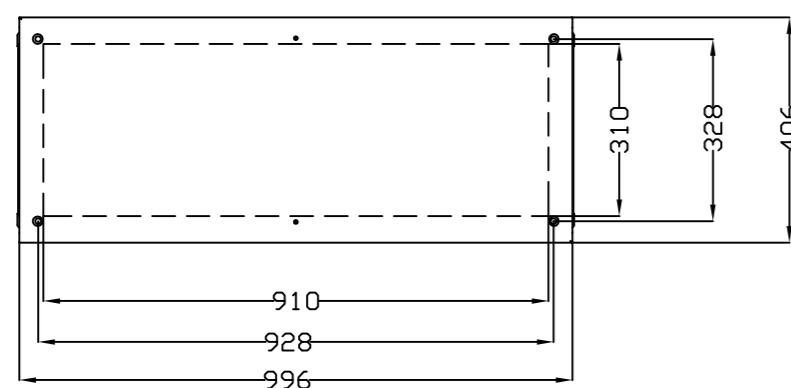
VISTA SUPERIOR TOP VIEW
