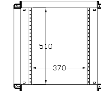
SEC. C-C
