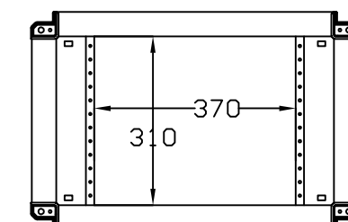
SEC. C-C
