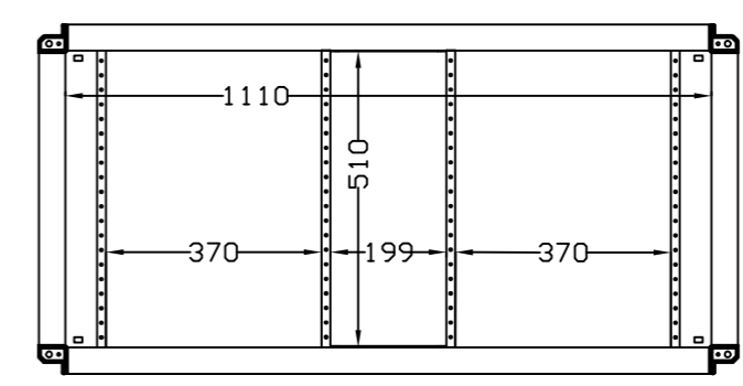
SEC. C-C
