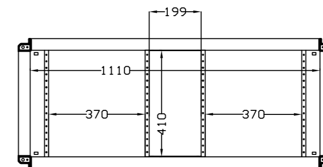
SEC. C-C
