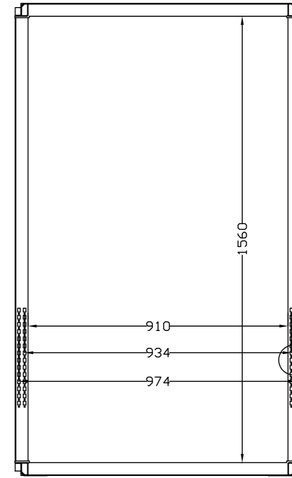
SEC. B-B
