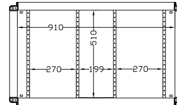
SEC. C-C
