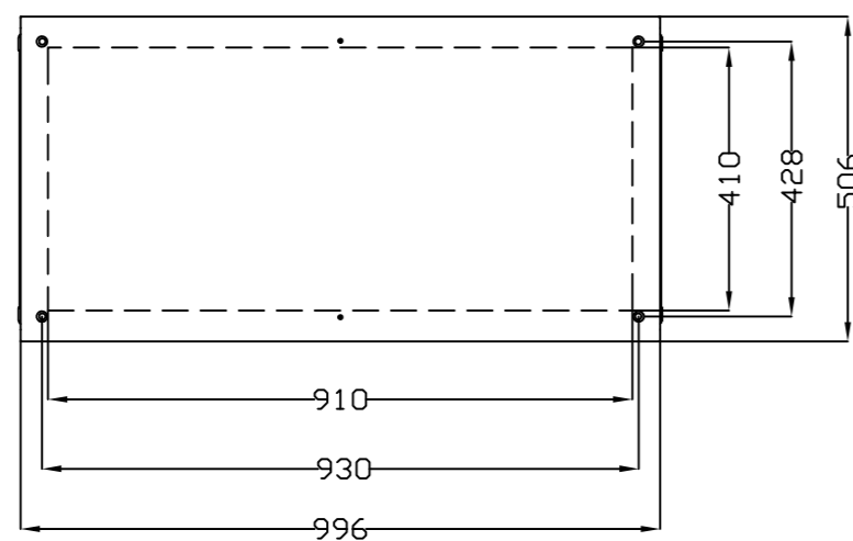
VISTA SUPERIOR TOP VIEW
